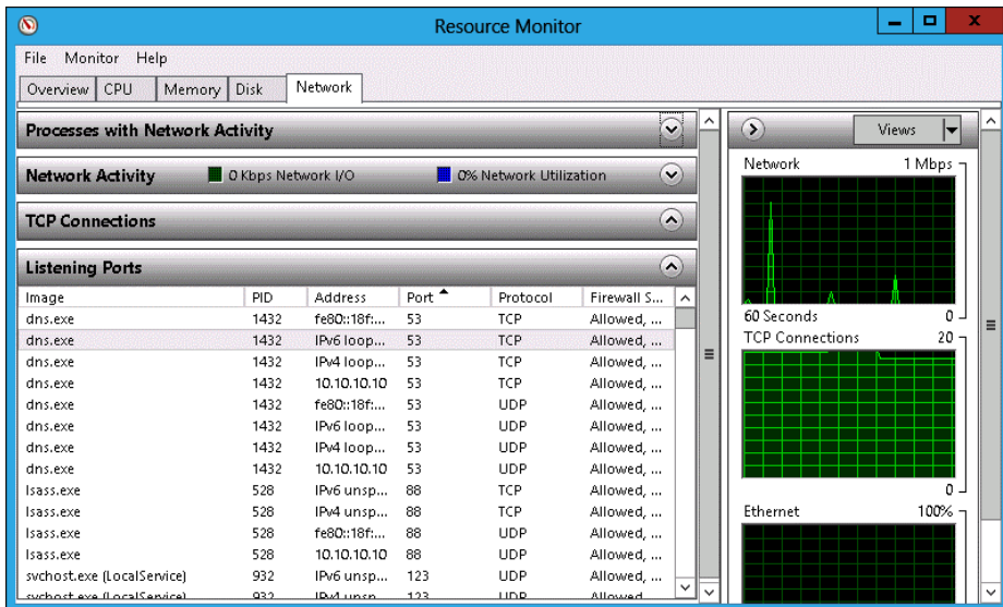
FIGURE 10-46 Listing the different ports.
