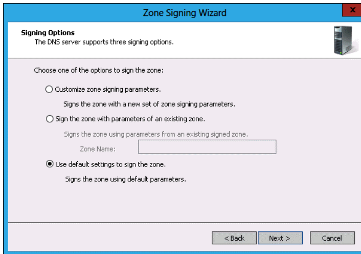
FIGURE 3-51 Sign DNS Zone
