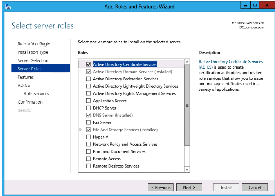
FIGURE 9-55 Adding an AD CS role
