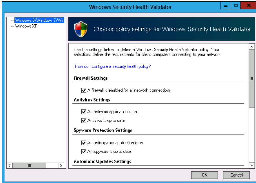
FIGURE 7-43 Configuring WSHV
