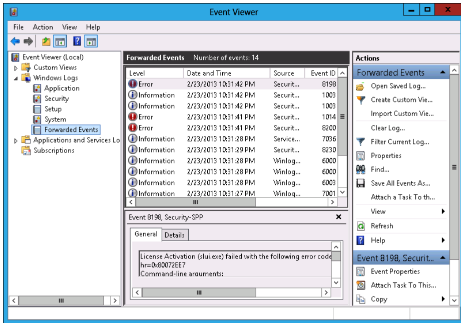
FIGURE 10-44 Event log
