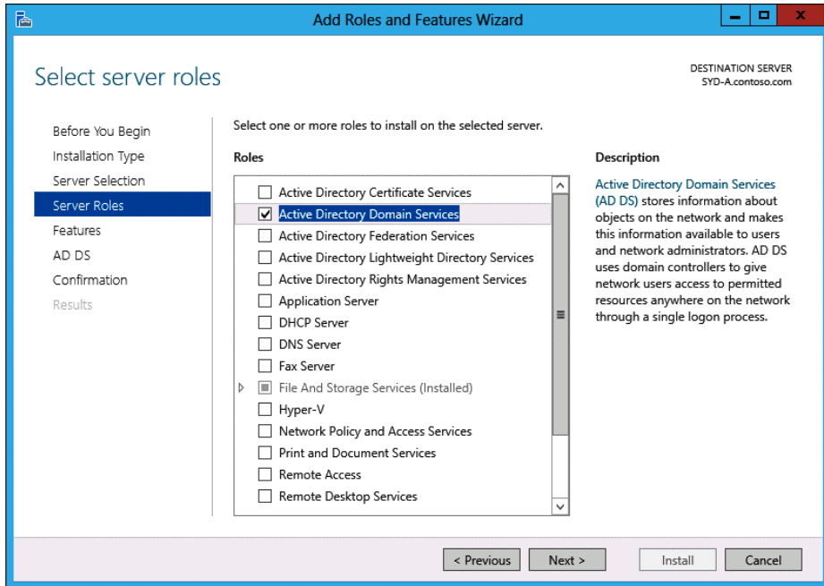
FIGURE 4-31 Adding the Active Directory Domain Services role
