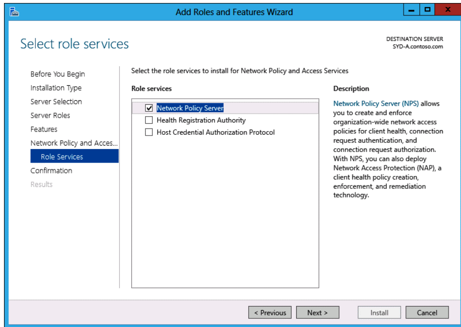
FIGURE 7-51 Selecting NPS role service
