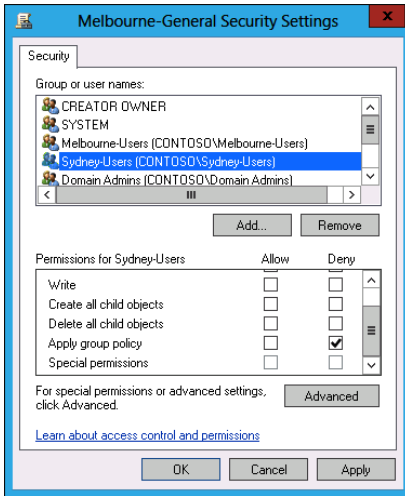
FIGURE 5-15 Security filtering
