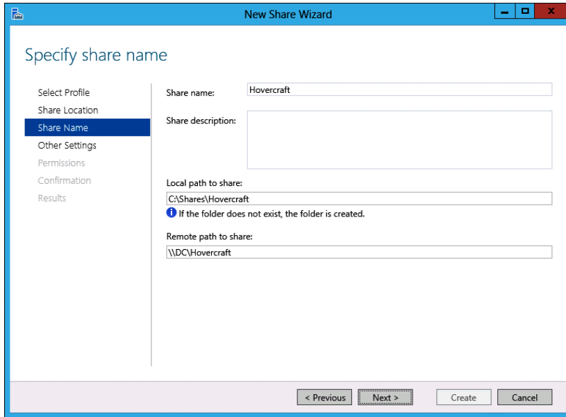
FIGURE 9-23 Share settings
