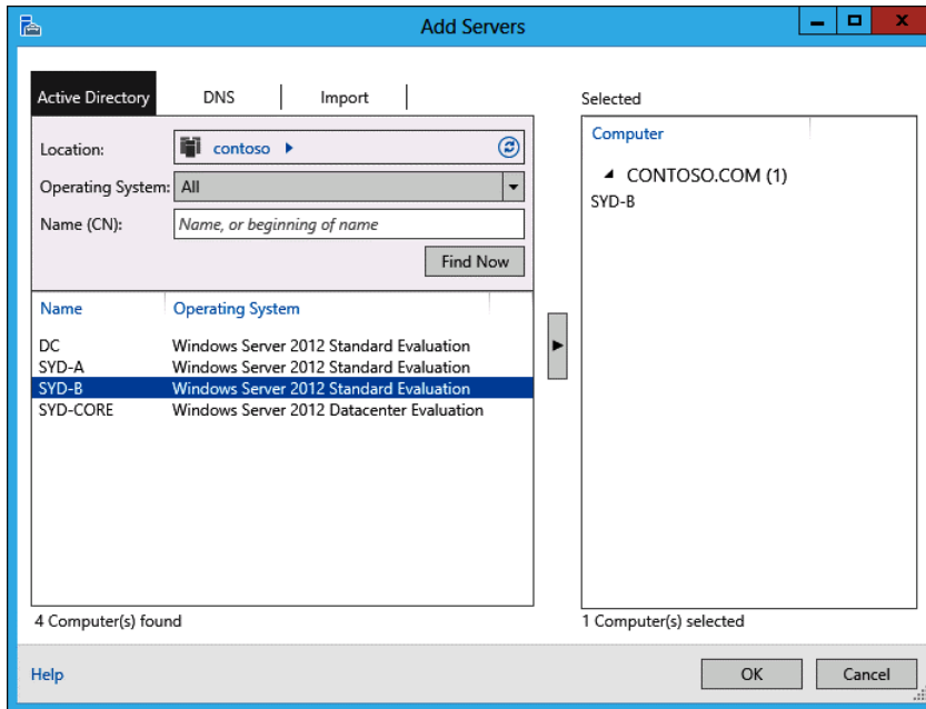
FIGURE 4-37 Adding servers
