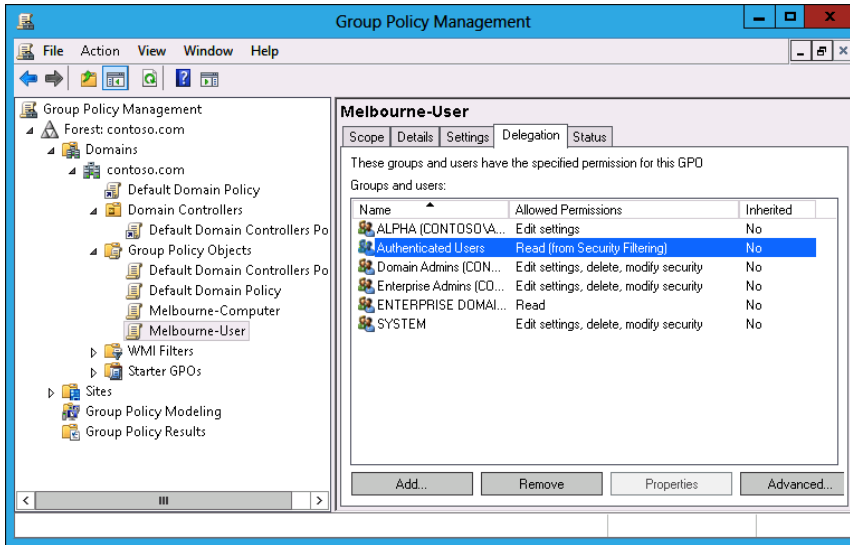
FIGURE 5-9 Delegating permissions
