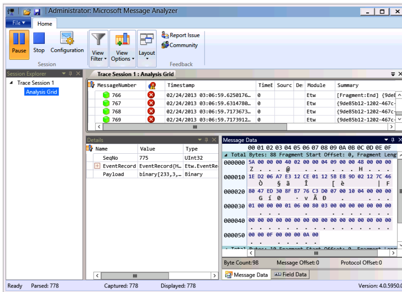
FIGURE 10-20 Message Analyzer
