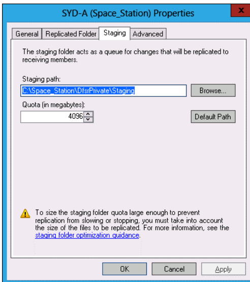
FIGURE 9-9 Staging folder
