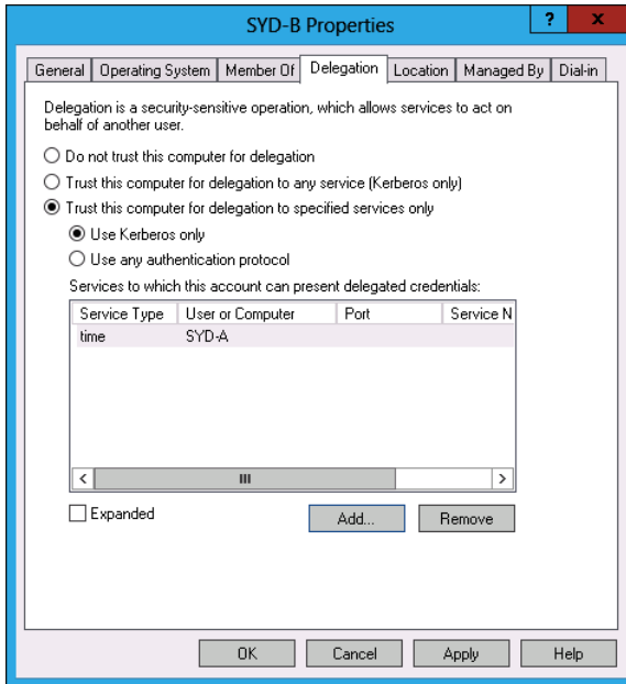
FIGURE 2-17 Kerberos delegation
