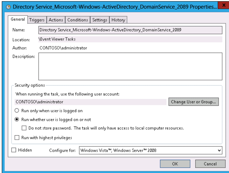
FIGURE 10-17 Run your task if the user is logged on or off
