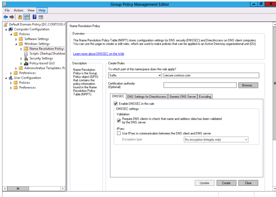
FIGURE 3-26 NRPT policy
