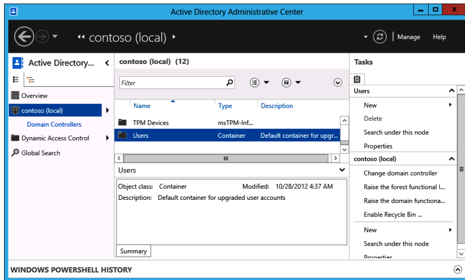
FIGURE 5-23 Users container
